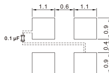
Footprint (Recommender)
