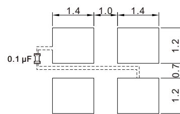
Footprint (Recommender)
